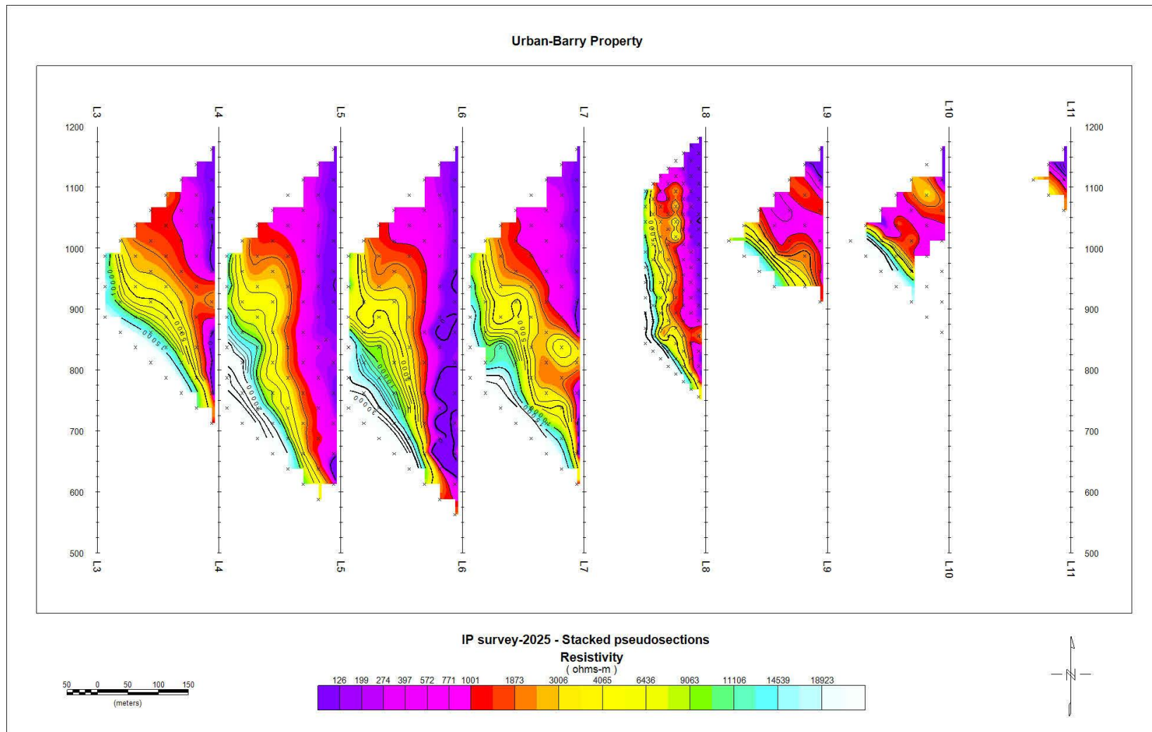
Figure 12 2025 IP Survey – Stacked Resistivity Pseudosections
