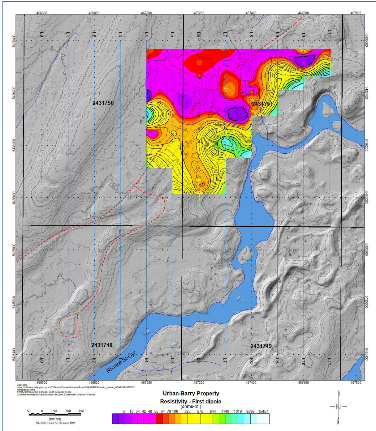
Figure 10 2025 Induced Polarisation Survey – First Dipole Resistivity
