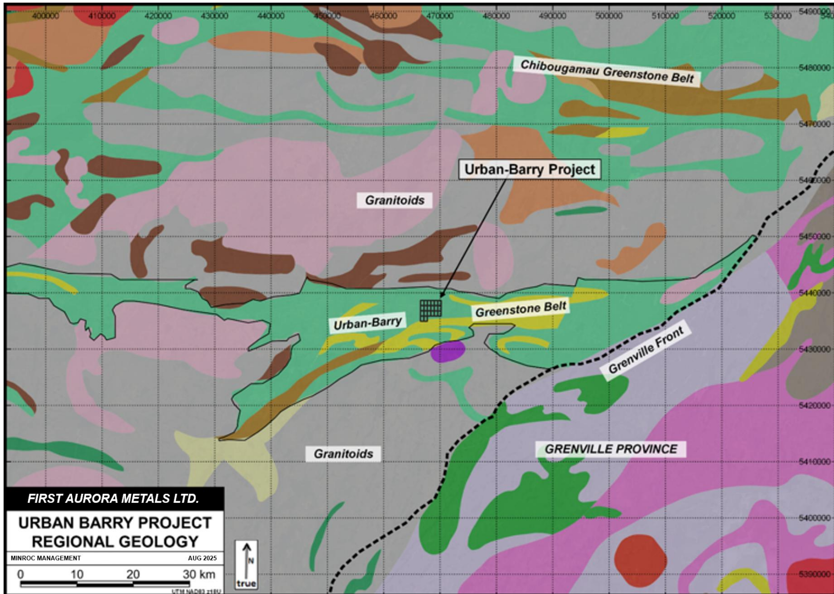
Figure 6 Regional Geology of the Urban Barry Property
