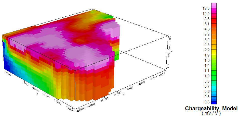
Figure 15 2025 Urban Barry IP survey - Chargeability Model.
