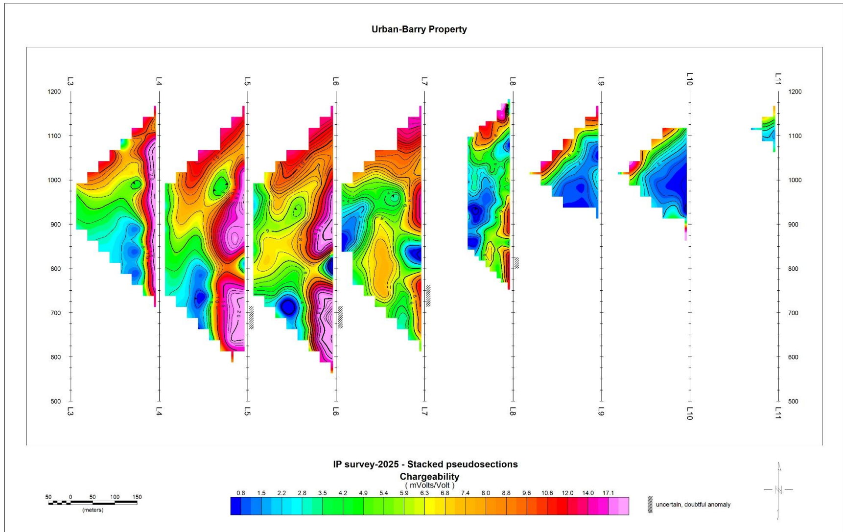
Figure 13 2025 IP Survey – Stacked Chargeability Pseudosections.
