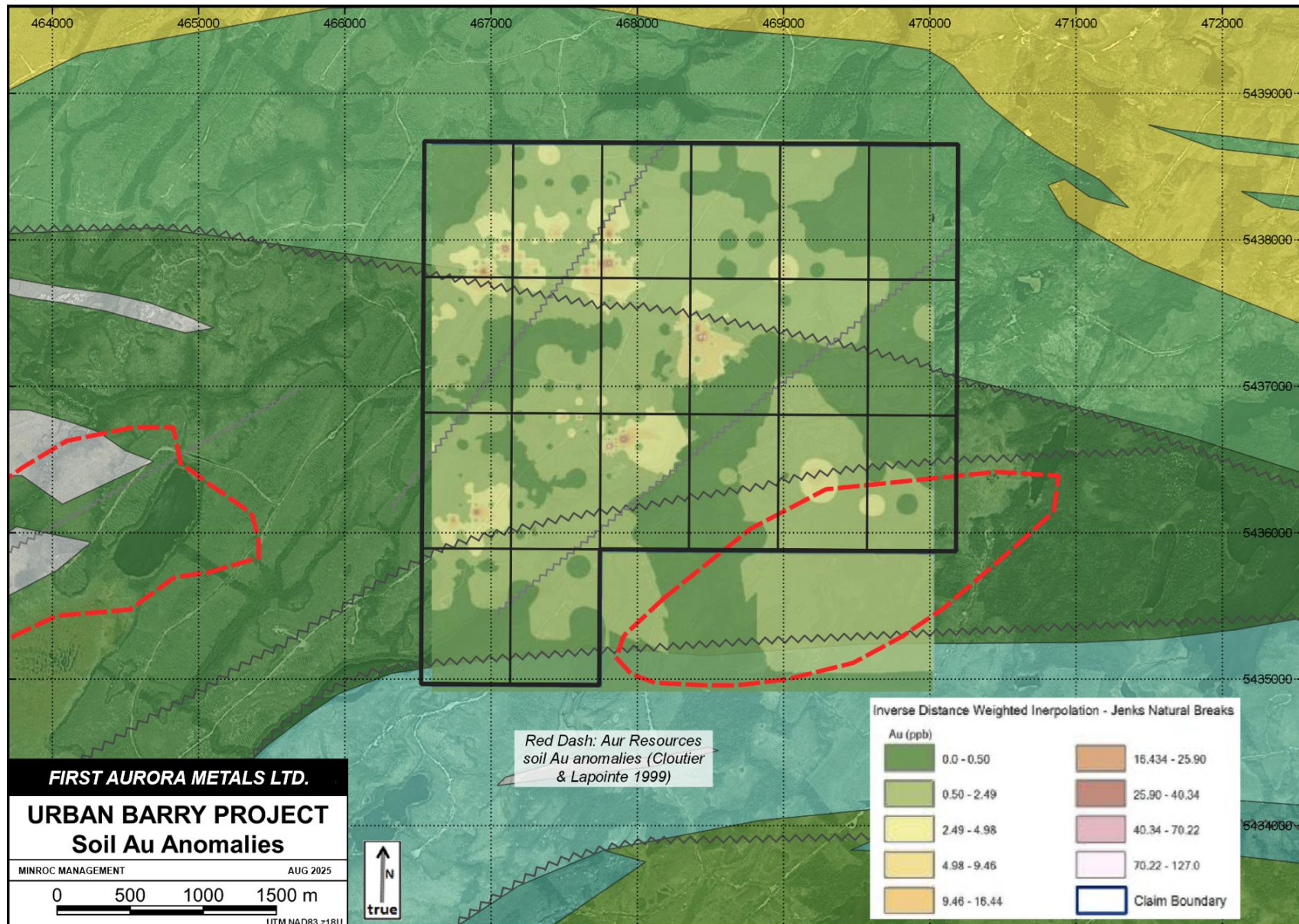
Figure 5 Gold-in-soil data from Aldever (Peterson 2017) and Aur Resources. Background from Property Geology (see Figure 7)
