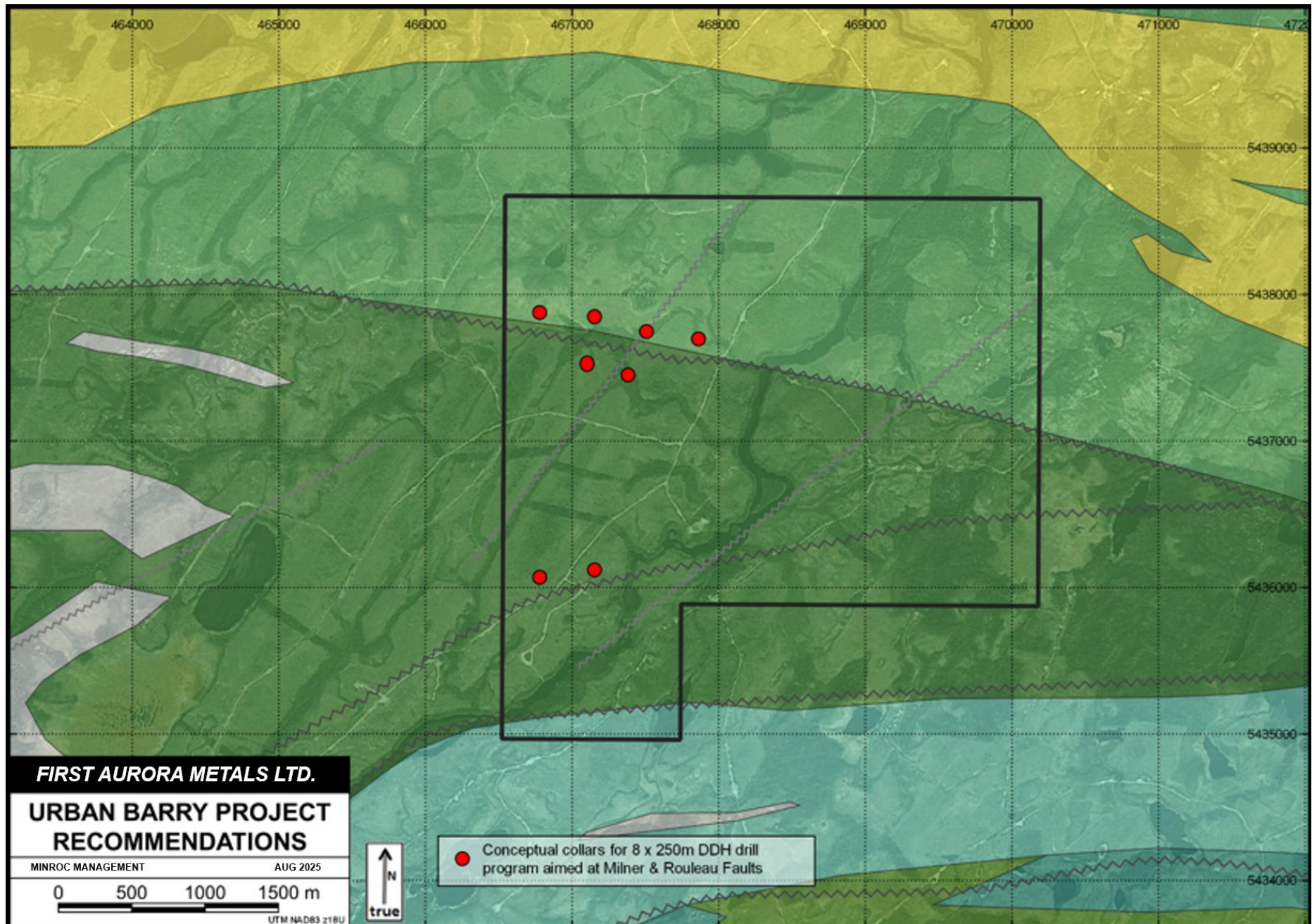
Figure 19 Map detailing the recommended work on the Urban Barry Property
