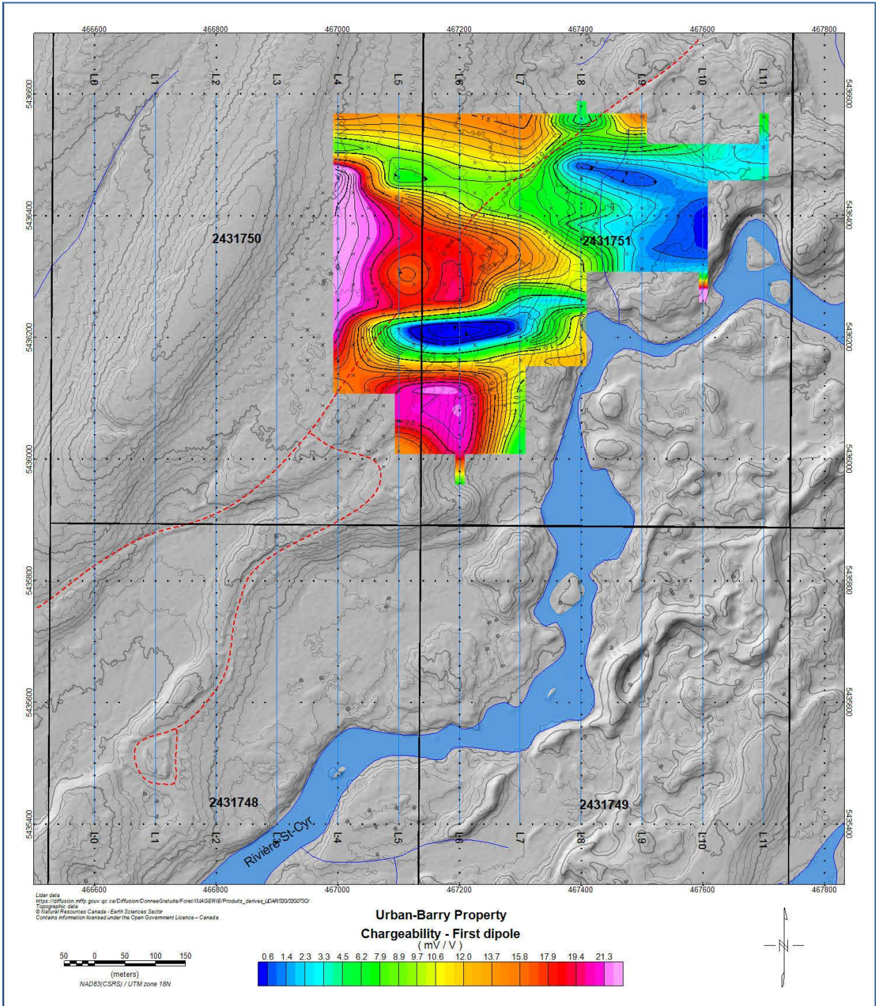
Figure 11 2025 Induced Polarisation Survey – First Dipole Chargeability.
