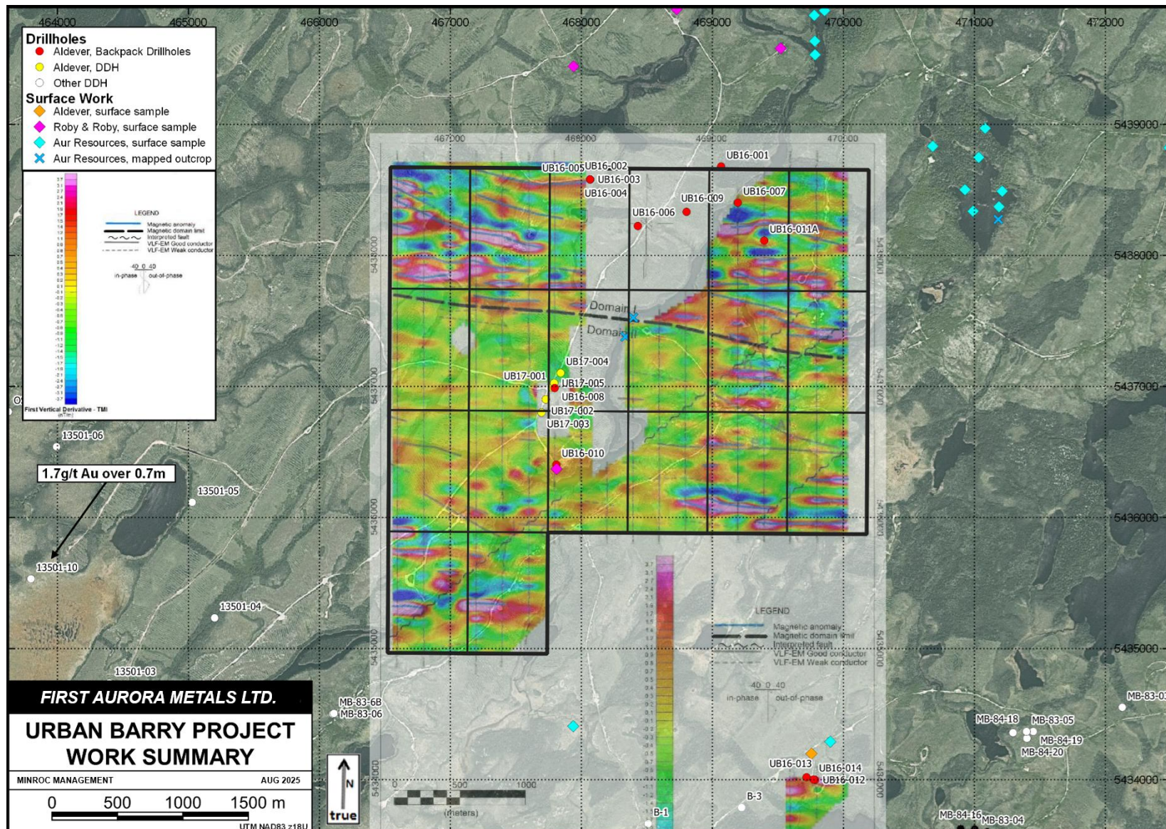
Figure 4 Historic Work Program Coverage at Urban Barry, showing Aldever VLF and magnetic data from Peterson (2017)
